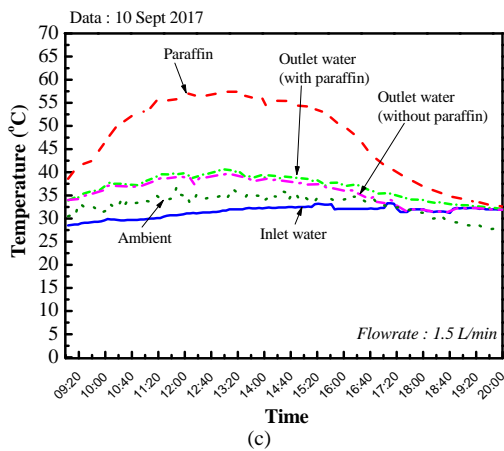
Figs. 5. Water, ambient and paraffin temperatures
