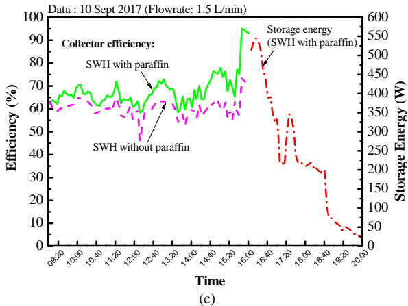
Figs. 7. Collector efficiency of SWH with V-shaped absorber plate with and without paraffin
