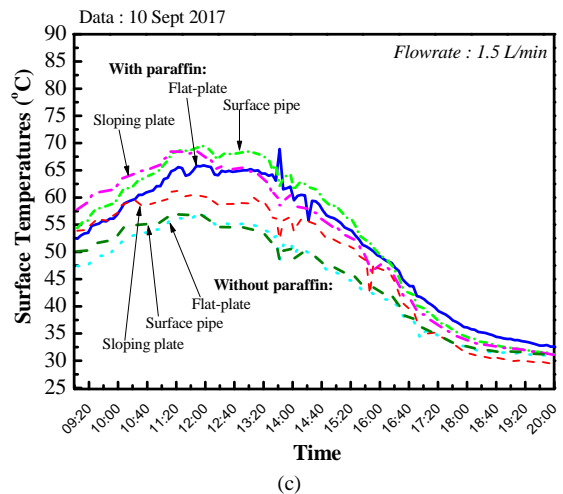
Figs. 6. Surface temperature of absorber plate on collector with paraffin and without paraffin
