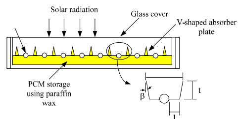
Fig. 1. V-shaped absorber plate integrated with PCM storage
