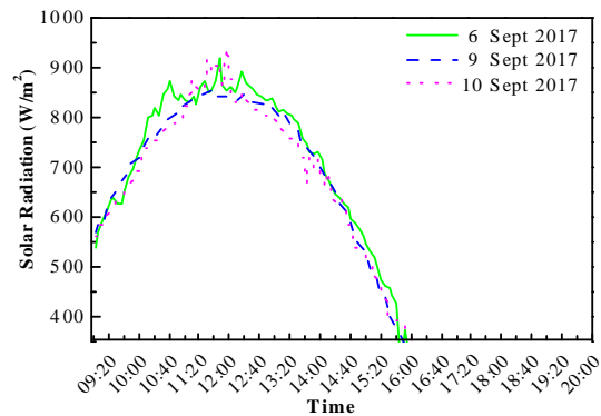
Fig. 4. Solar Radiation
