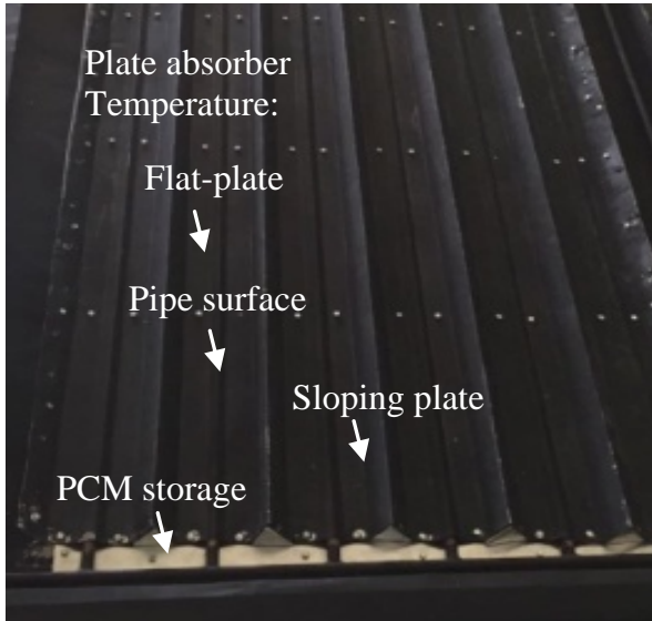
Fig. 3. V-shaped absorber plate with PCM storage
